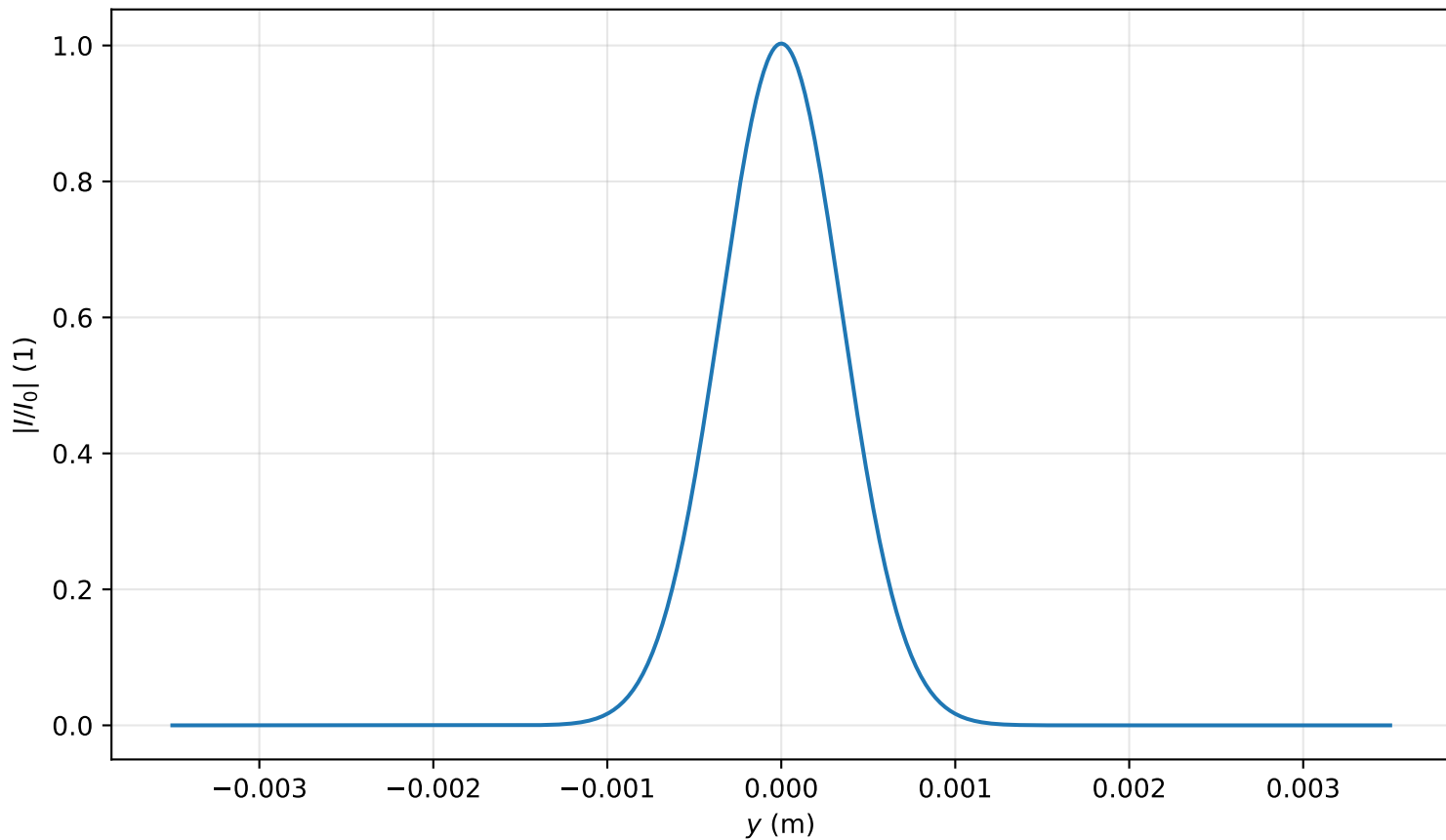
Intensity profile I(x=0, y, z=0.080)/I_0 , P_{in}=0.7P_{cr} , artificial time
